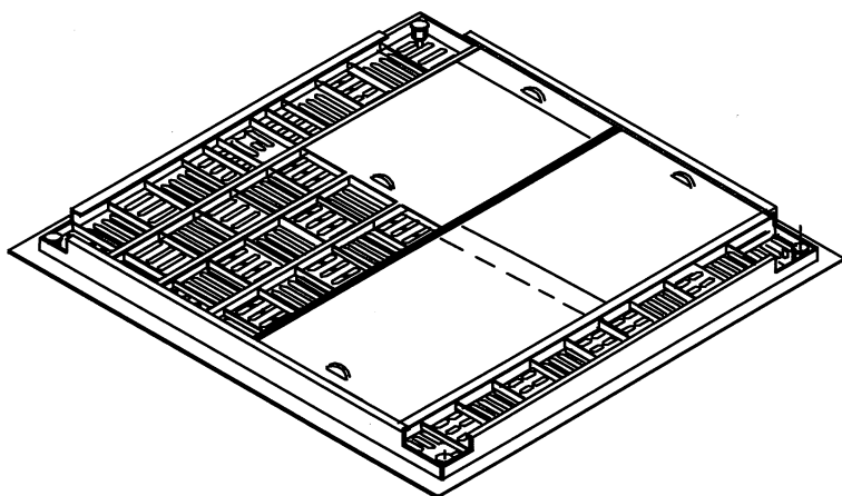
Example of Quad Slide Damper in 3/4 closed position
